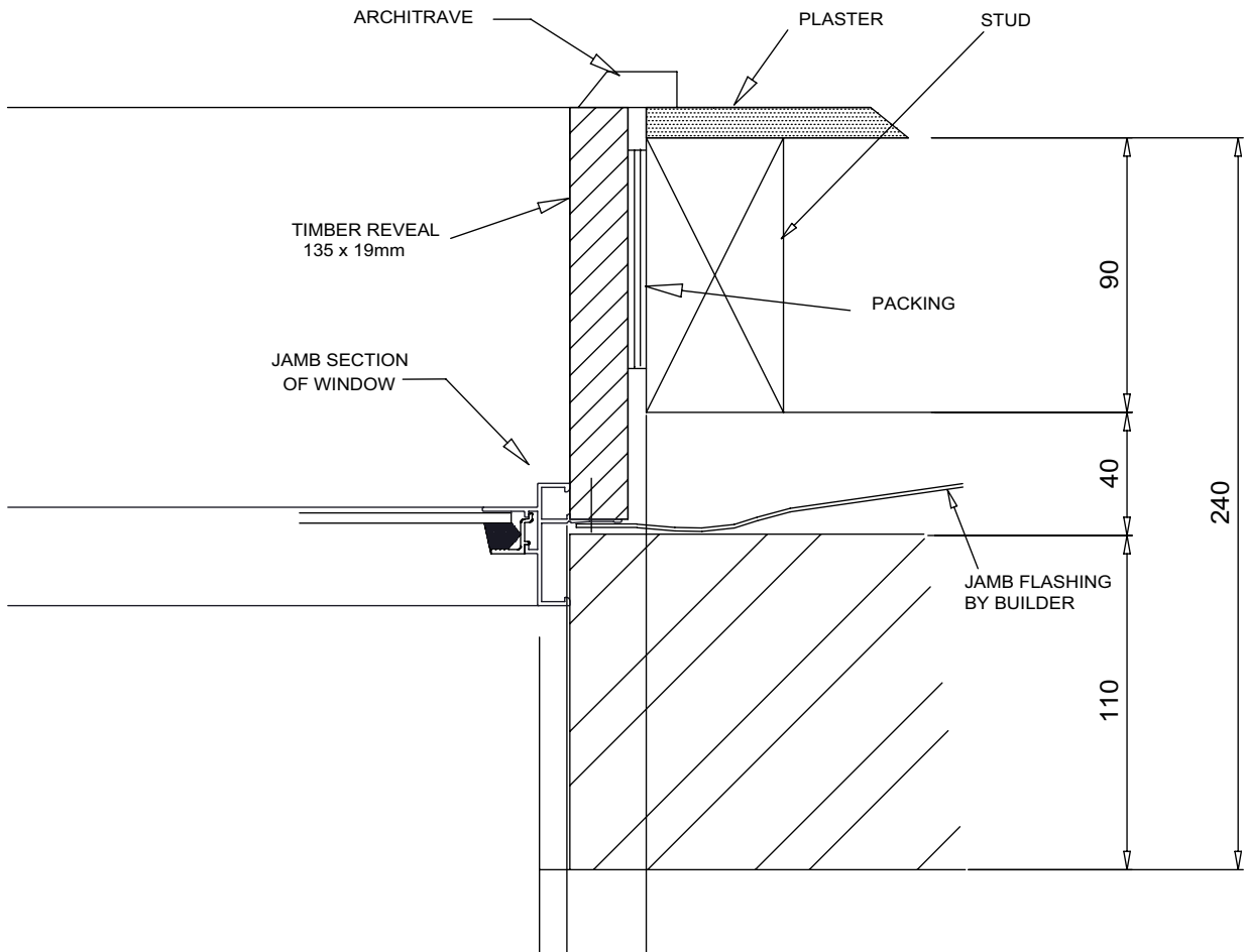
TYPICAL JAMB DETAIL
