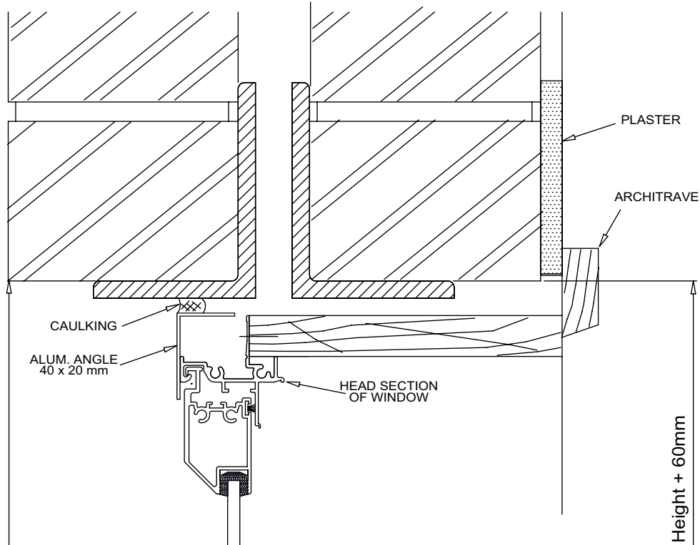
TYPICAL HEAD DETAIL
