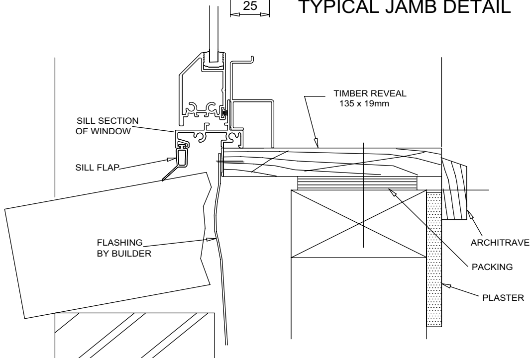
TYPICAL SILL DETAIL
