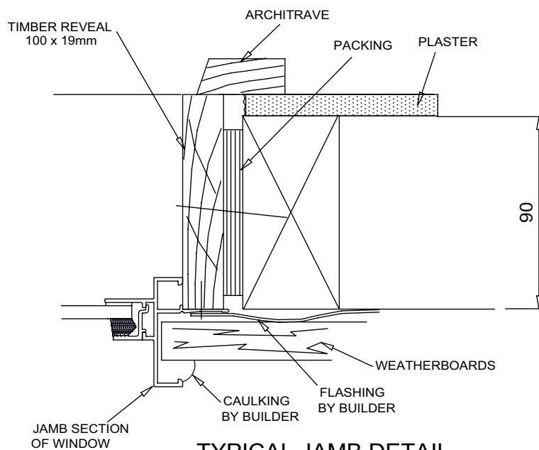
TYPICAL JAMB DETAIL
