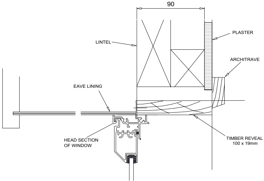
TYPICAL HEAD DETAIL (EAVES OVER WINDOW)
